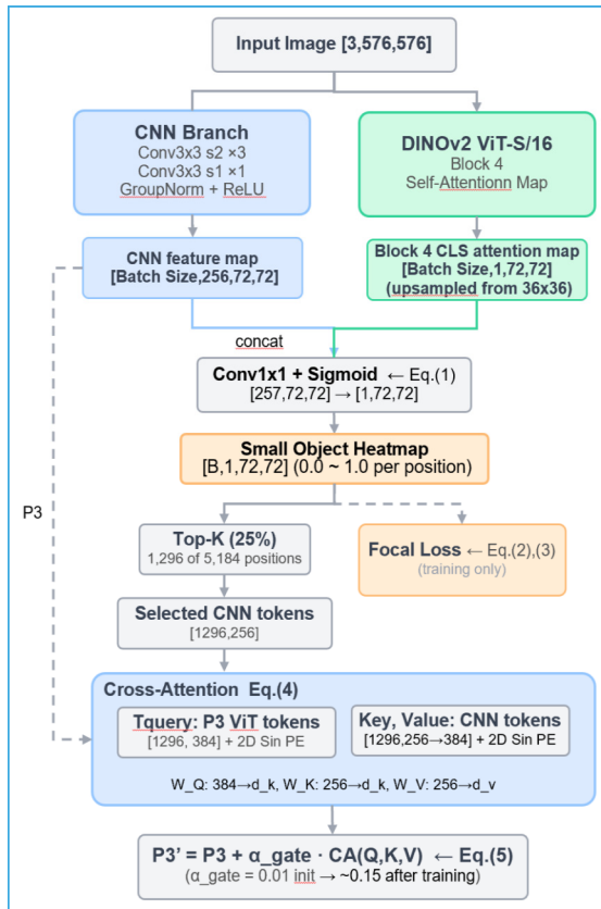
Figure 2. Architecture of the SCA module
