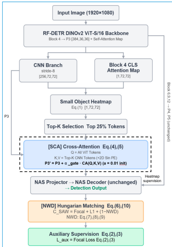
Figure 1. Pipeline of the proposed small object detection
