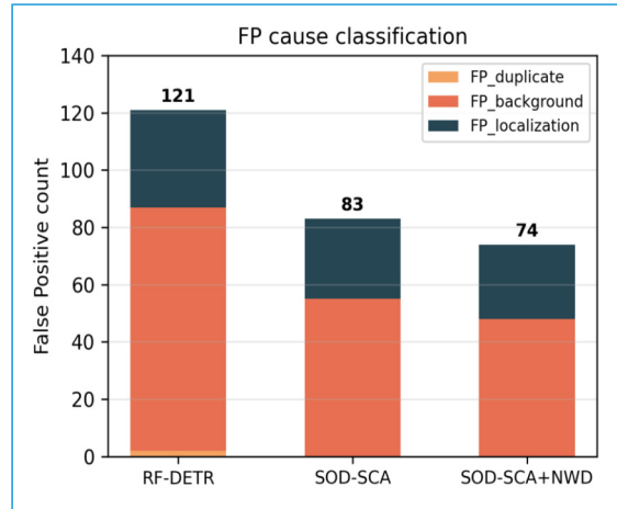
Figure 4. FP cause classification by experiment configuration
