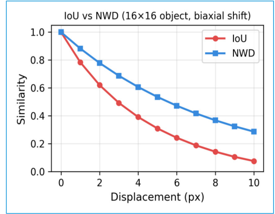
Figure 3. IoU and NWD response comparison
